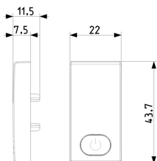
09021.S.CM - Button 1M switch ON symbol carbon matt
